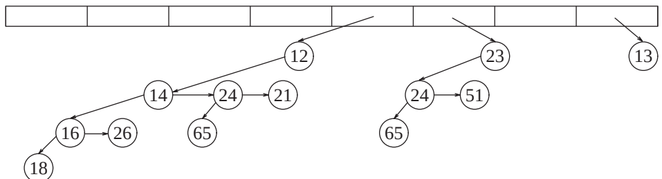
Figure 6.51 Representation of binomial queue H_3
