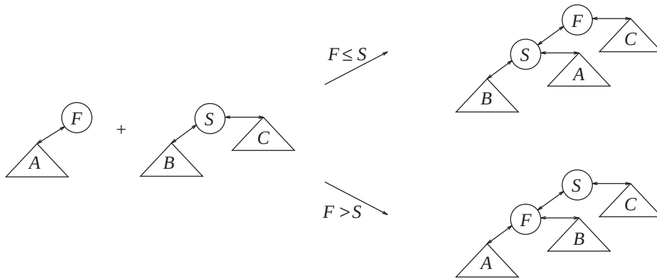
Figure 12.44 compareAndLink merges two subheaps
