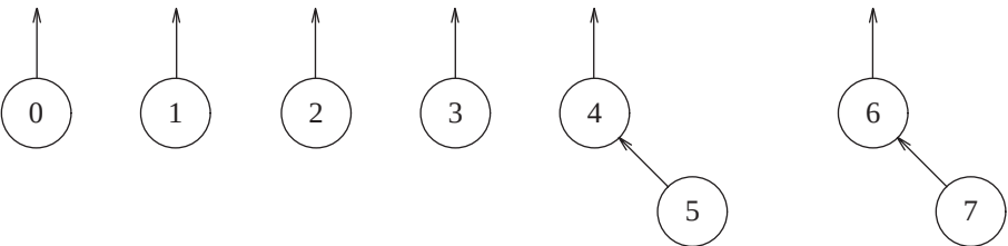
Figure 8.3 After union(6,7)
